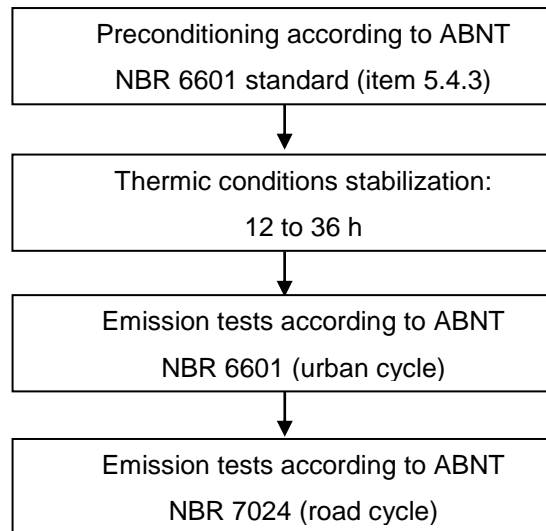
Figure 1- Measurement activities flow chart of the Proficiency Testing
