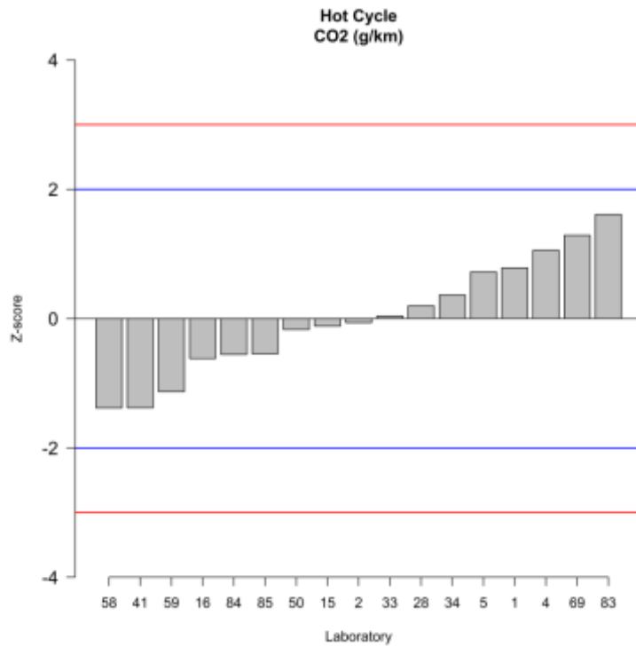
Figure 33 – z-score graph for CO 2 measurement – Hot Cycle
