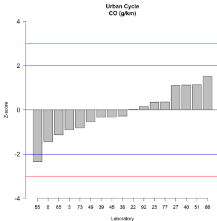
Figure 22 – z-score graph for CO measurement – Urban cycle
